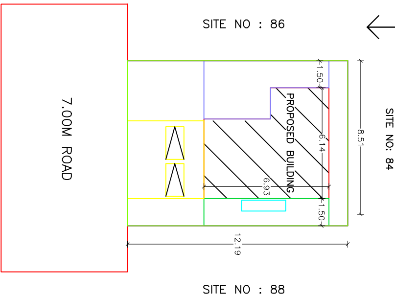
SITE PLAN
