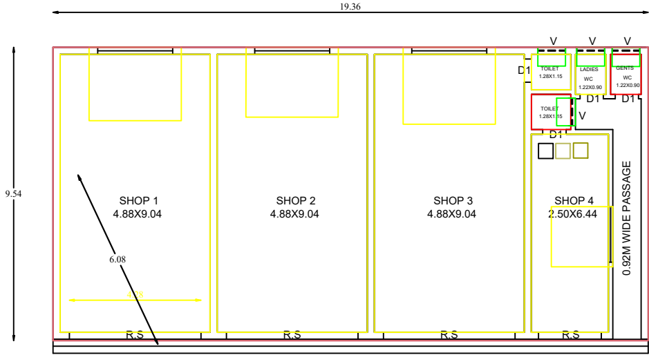
GROUND FLOOR PLAN SCALE 1 CM = 1 M
