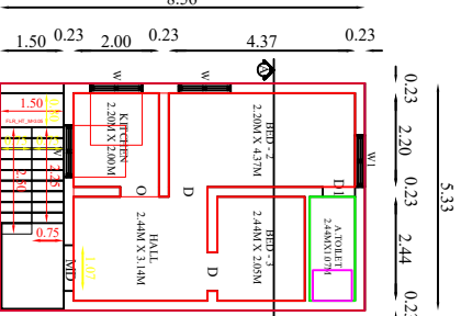
PROPOSED FIRST FLOOR PLAN
