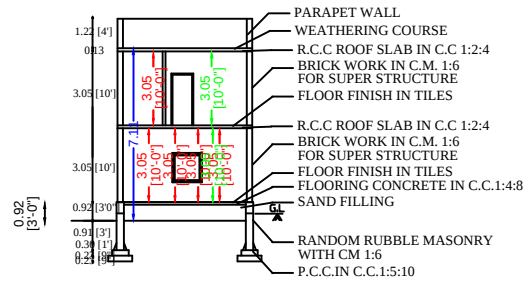
Section On "PS"
