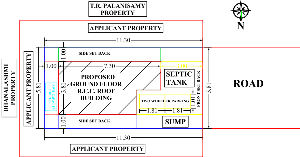
SITE PLAN
