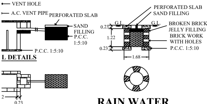
ANK DETAILS
