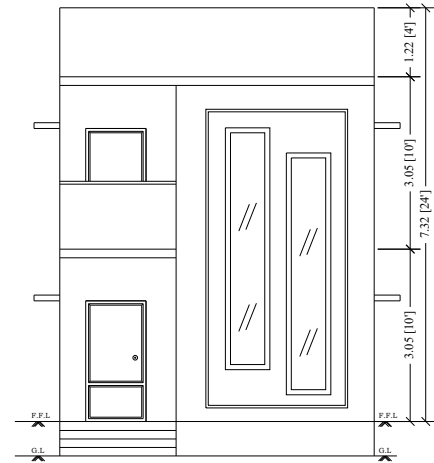
FRONT ELEVATION
