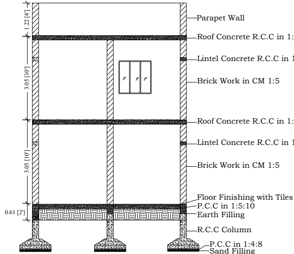
SECTION X-X
