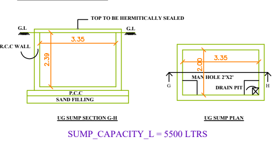
UG SUMP DETAILS
