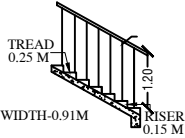
STAIRCASE DETAILS
