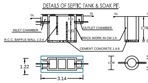
DETAILS OF SEPTIC TANK & SOAK PIT
