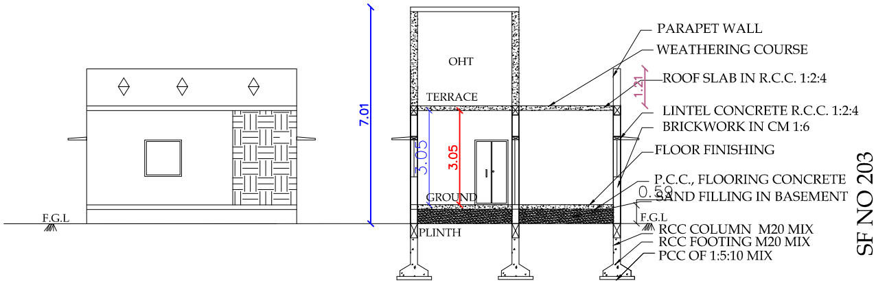
ELEVATION-VIEW A
