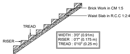
STAIRCASE DETAILS
