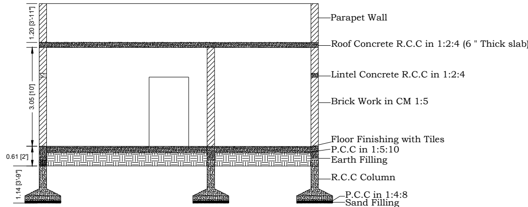
SECTION X-X
