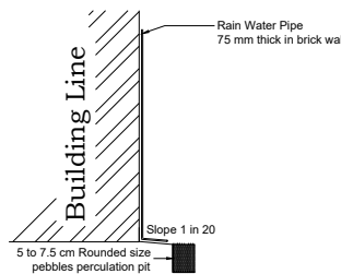
RAINWATER HARVESTING
