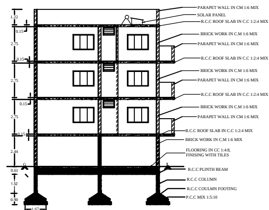
SECTION "A-B"
