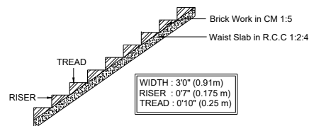
STAIRCASE DETAILS
