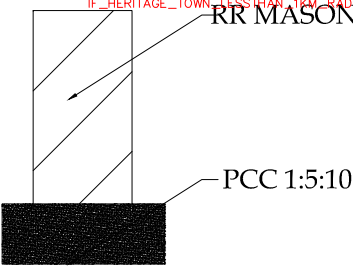
FOUNDATION DETAIL
