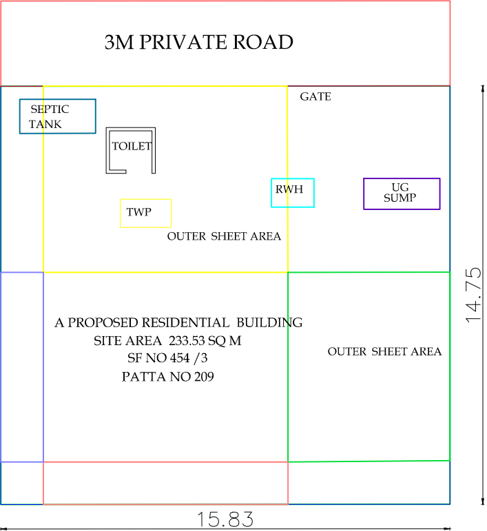
SITE PLAN
