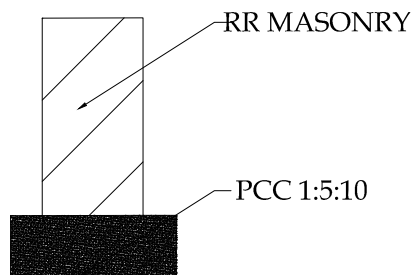
FOUNDATION DETAIL
