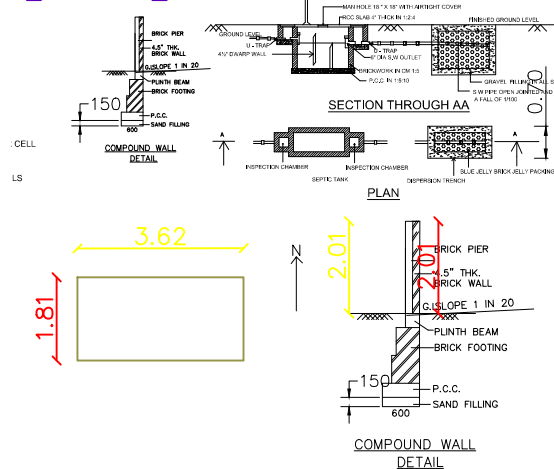
FOUNDATION DETAIL
