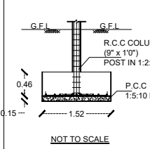
COLUMN POST DETAILS
