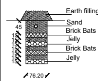
SECTION ON B-B.
