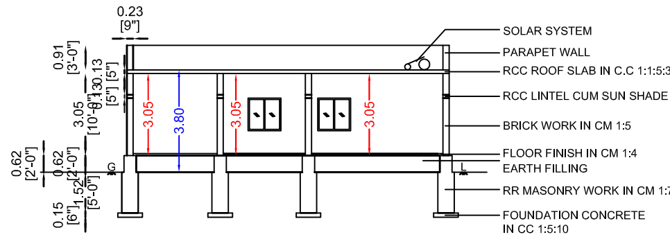
SECTION "AB"
