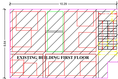
FIRST FLOOR EXISTING PLAN
