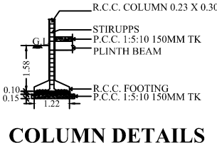
COLUMN DETAILS
