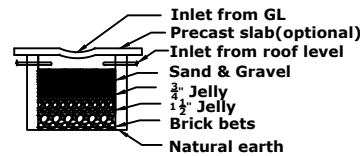
sectional elevation
