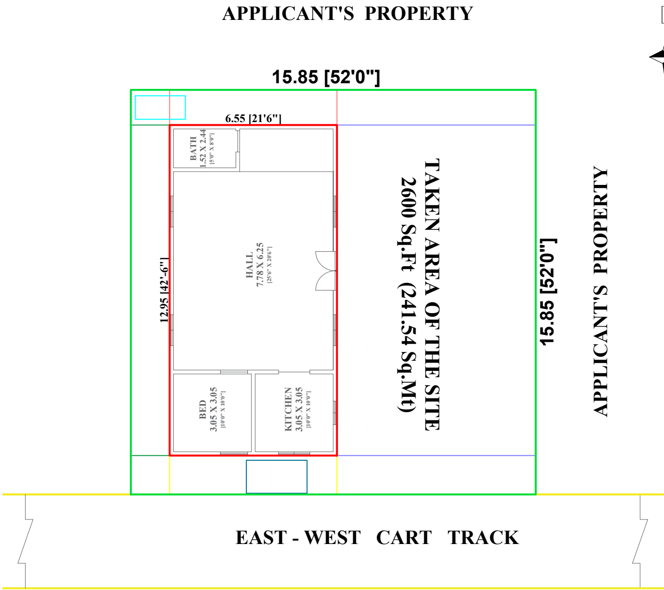
SITE PLAN
