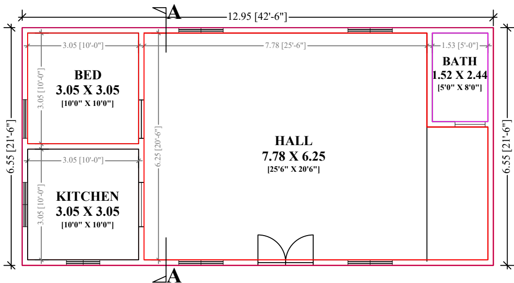
BUILDING PLAN
