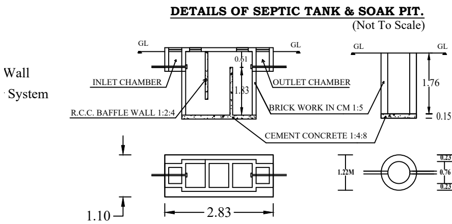
SECTION
