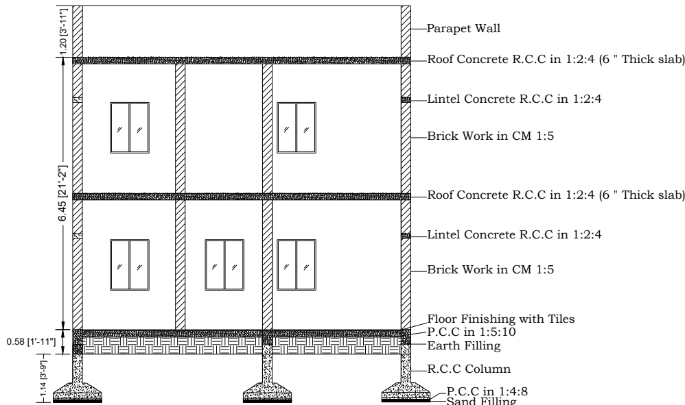
SECTION X-X
