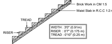
STAIRCASE DETAILS
