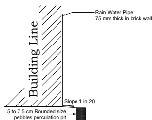
RAINWATER HARVESTING
