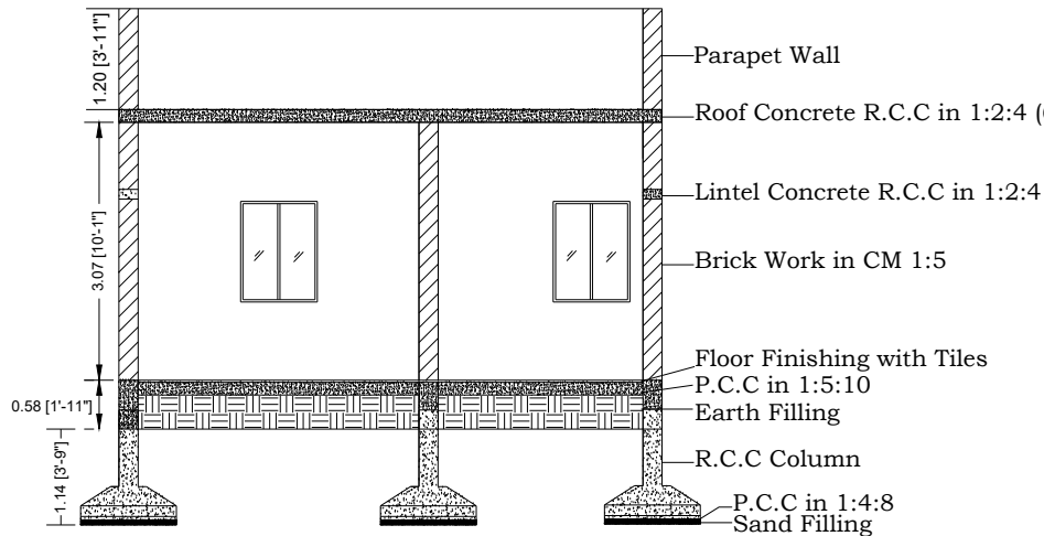
SECTION X-X
