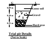
Trial pit Details (Not to Scale)
