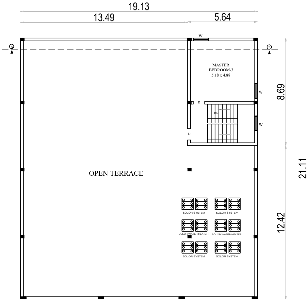
FIRST FLOOR RCC PLAN
