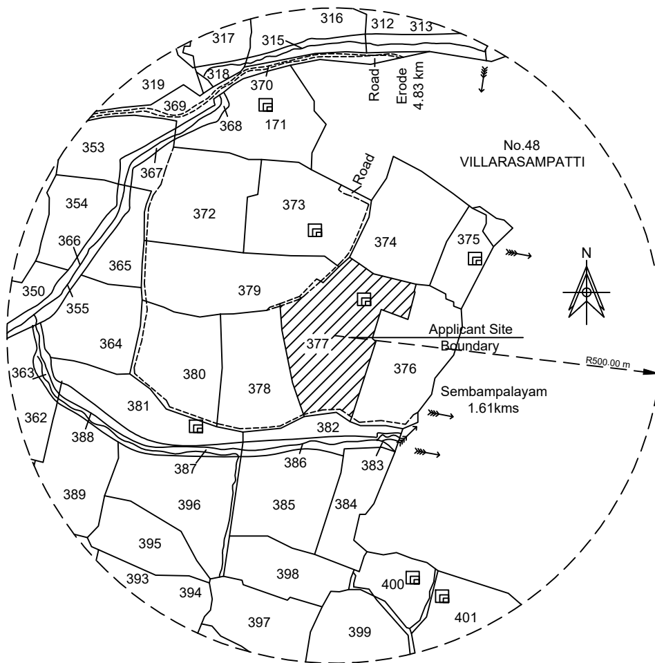
TOPO PLAN
