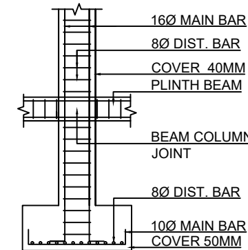
TYPICAL FOOTING COLUMN AND BEAM
