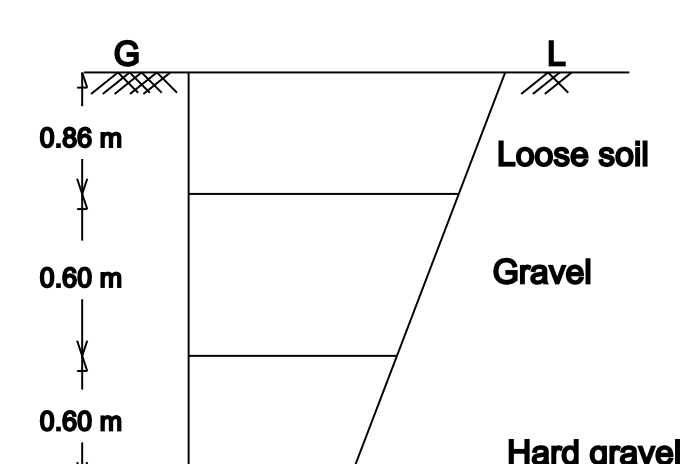
Trial pit Details (Not to Scale)
