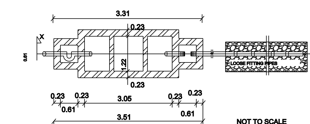
SEPTICK TANK & DISPERSION TRINCH
