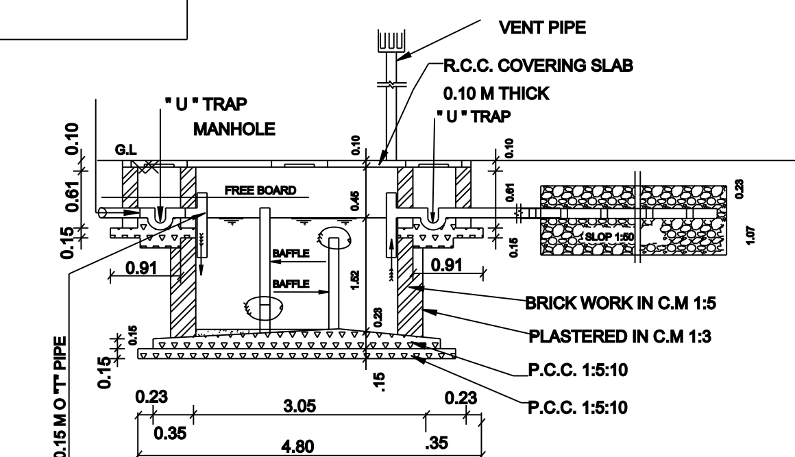
LONGITODINAL SECTION IN "XX"
