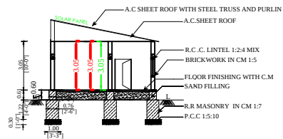
SECTION ON "JM"
