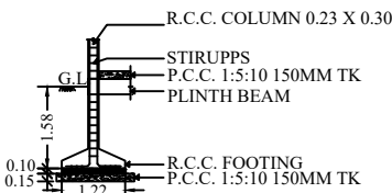
COLUMN DETAILS
