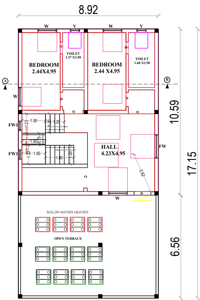
FIRST FLOOR RCC PLAN
