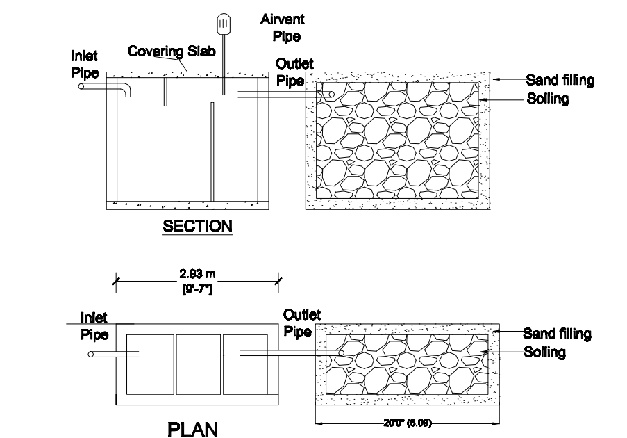
DETAILS OF SEPTIC TANK & DISPERSION TRENCH
