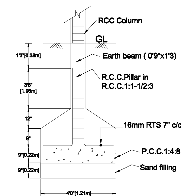
FOUNDATION DETAILS
