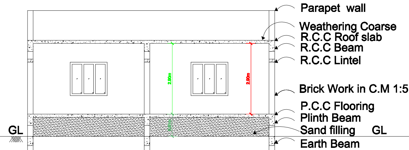
SECTION ON "RR"
