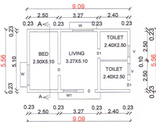
PLAN OF GROUND FLOOR BLOCK:1 R.C.C.ROOF
