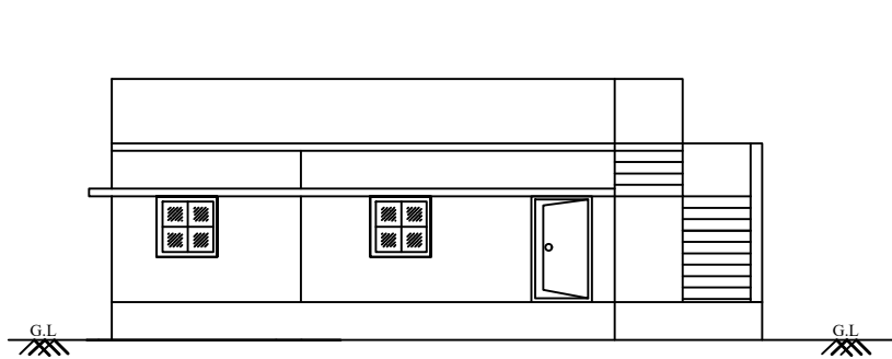
FRONT FACE ELEVATION
