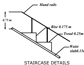
STAIRCASE DETAILS
