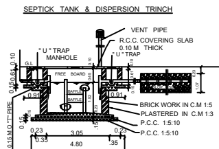
SEPTICK TANK & DISPERSION TRINCH
