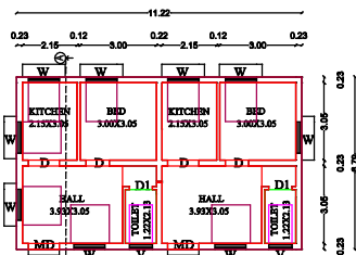
PROPOSED CEILING PLAN
