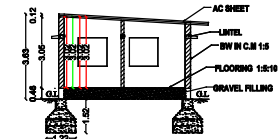
SECTION ON "AA"
