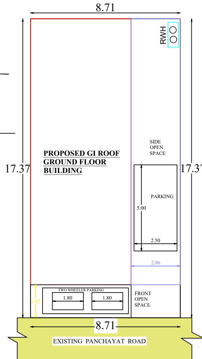
SITE & LOCATION PLAN SCALE - 1: 100
