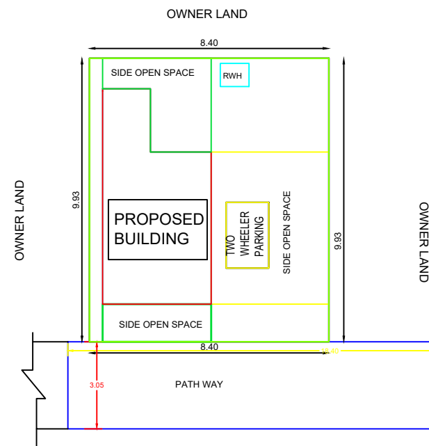
SITE PLAN
