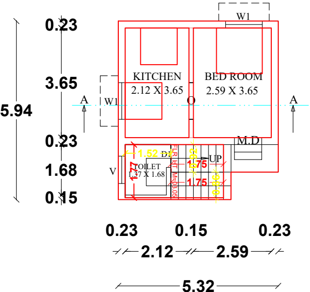
GROUND FLOOR PLAN ( East Facing )
