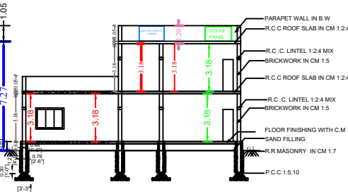
SECTION ON "JJ"
