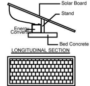
PLAN SOLAR SYSTEM Not To Scale
