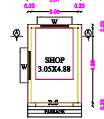
ADDI.PROPOSED GF.PLAN
