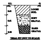
FOUNDATION DETAILS
