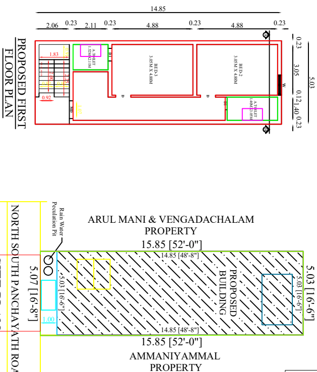
SITE PLAN
