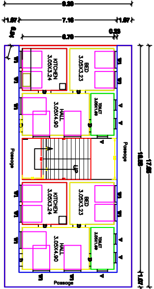
FIRST FLOOR PLAN (PROPOSED - RESIDENTIAL)
