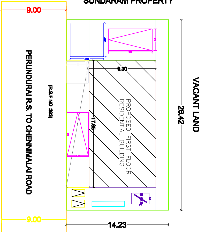
SITE PLAN
