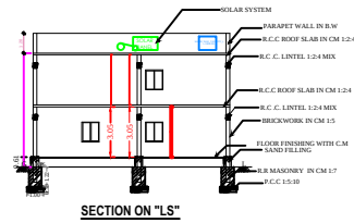
SECTION ON "LS"
