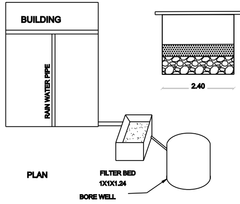
RAIN WATER HARVESTING TANK
