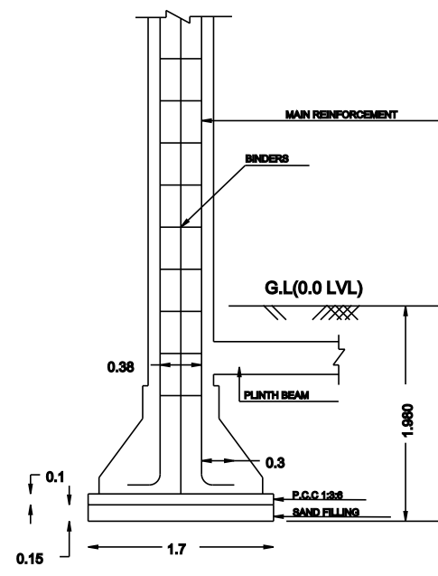
TYPICAL SECTION OF R.C.C COLUMN FOUNDATION
