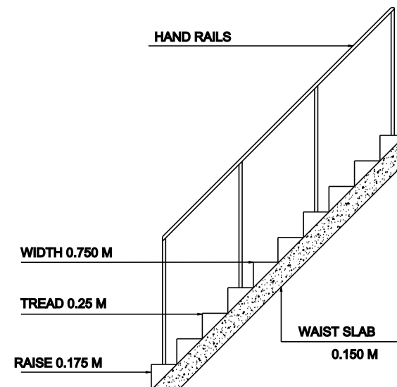
STAIRCASE DETAILS
