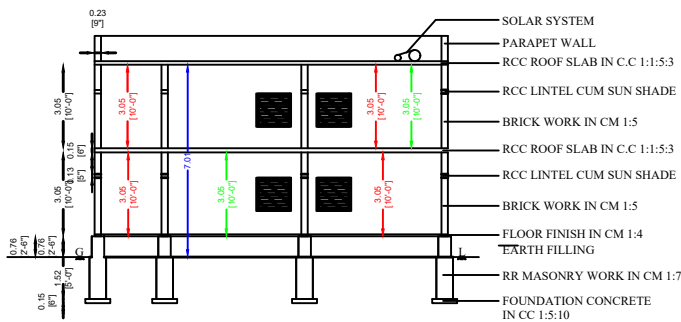
SECTION "AA","BB"
