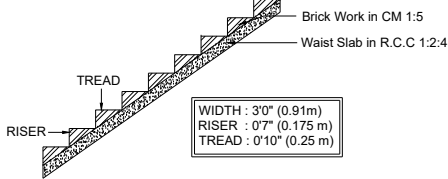
STAIRCASE DETAILS
