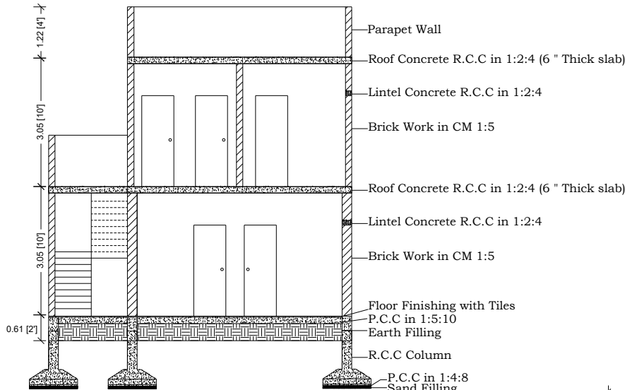
SECTION X-X
