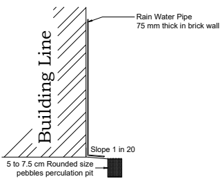
RAINWATER HARVESTING
