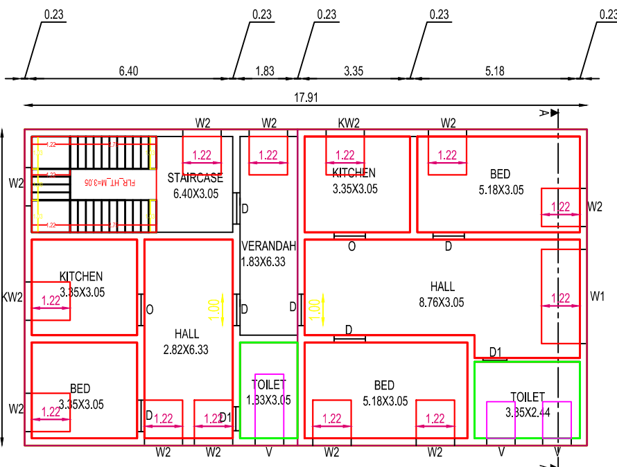
PRO.ADDL.FIRST FLOOR PLAN (Scale : 1:100)
