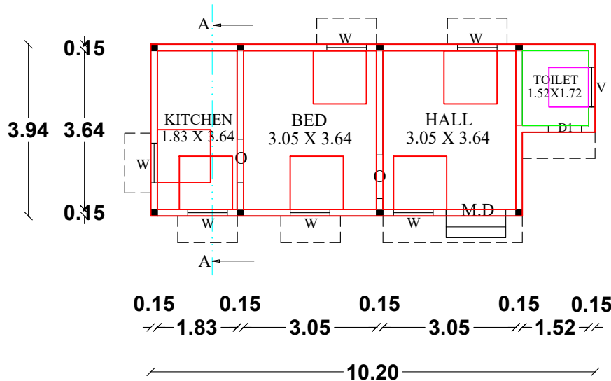
GROUND FLOOR PLAN ( East Facing )
