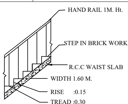
STAIR DETAIL
